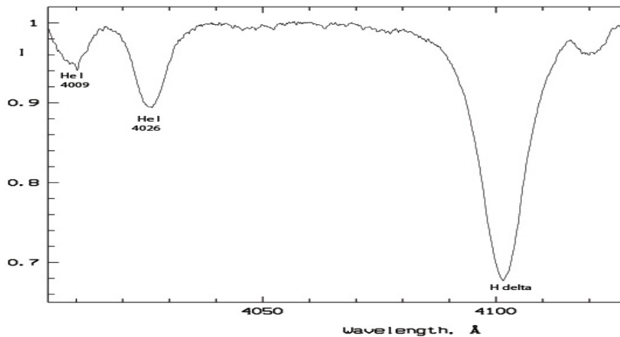
Figure 1: Fragment of a normalized spectrum of HD 182180 around H \delta (averaged over 11 frames)
