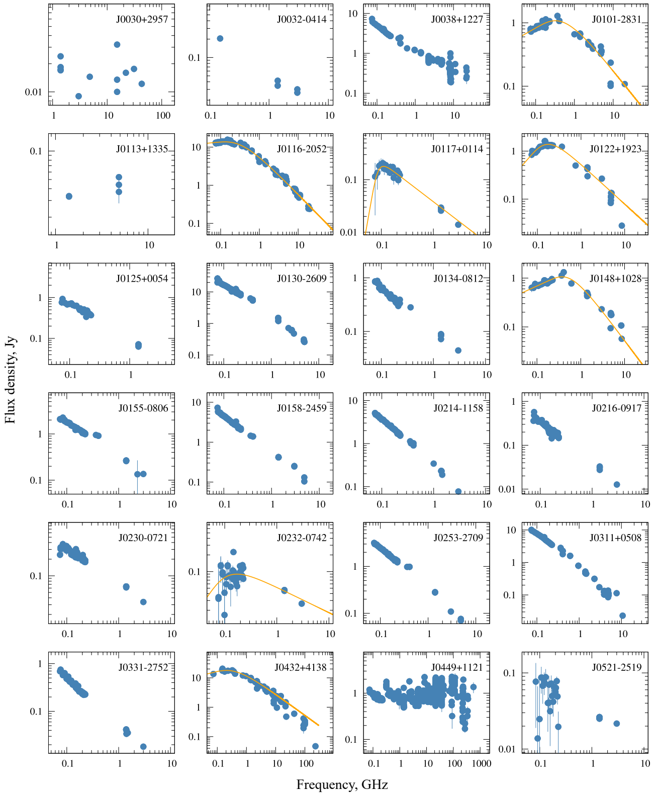
Fig. 3. The radio continuum spectra of the galaxies.
